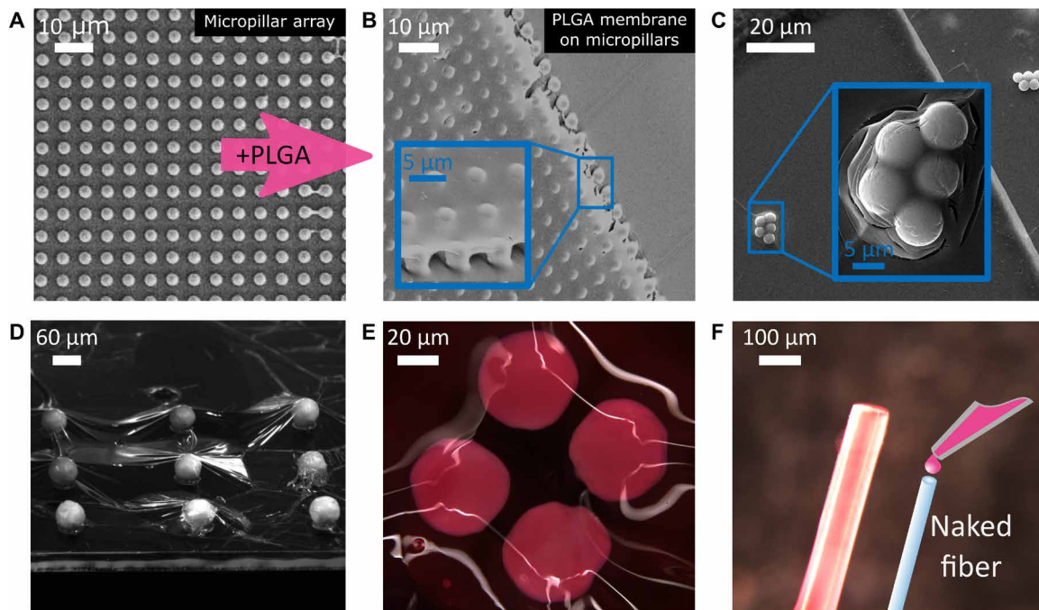
Fig. 4. Polymer packaging of micropillars, macroarray, and optical fiber. (A) SEM image of micropillar array (top view) and (B) corresponding SEM image of polymer membranes suspended over the micropillar structure. (C) Packaging of five latex microspheres. The difference between coated (left) and uncoated (right) microspheres is evident. (D and E) Side view and top view of water packaging for a matrix of microspheres submerged in water. (F) Outline of polymer membrane formation directly onto the top of optical fiber and stereoscope image of the coating realized.
